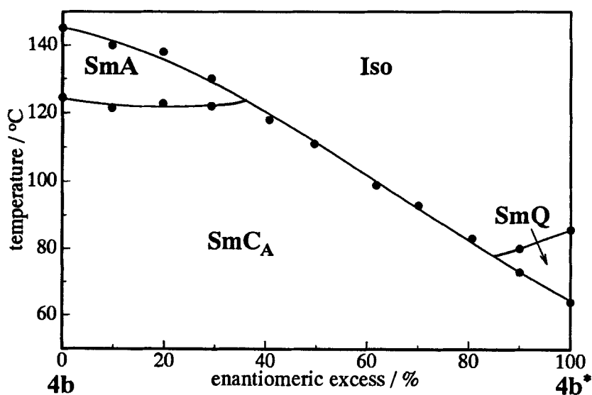
FIGURE 5 Chiral-racemic phase diagram of 4b * in 4b
