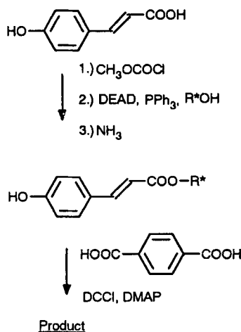
FIGURE 1 Synthesis scheme of series 3
