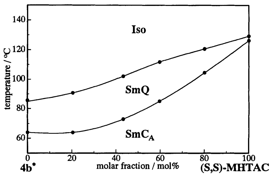
FIGURE 4 Phase diagram of (S,S)-MHTAC in 4b*
