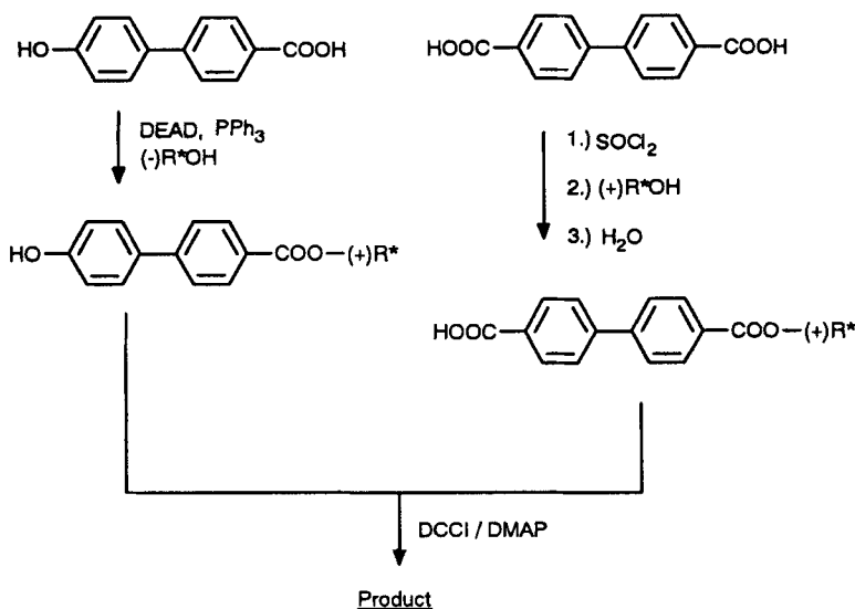
FIGURE 2 Synthesis scheme of series 4. Note that both enantiomers of the chiral alcohol are needed to get the (R,R) or (S,S) enantiomer of the product.
